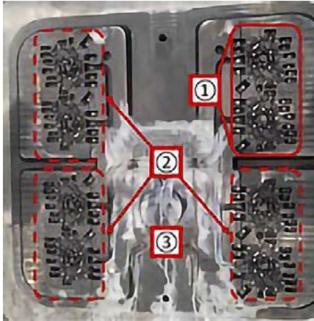
Fig. 7: HPDC tool assembly;
