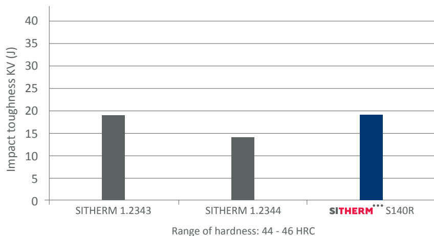
Fig. 1: Impact toughness
